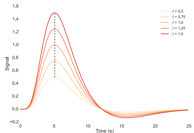
Figure 1. Standard canonical hemodynamic response function model of blood oxygen level-dependent activity. In regression-based approaches, it is assumed that the only way the blood oxygen level-dependent response is modulated is that the canonical shape is multiplied by some factor \beta .
